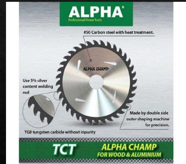
CIRCULAR SAW
